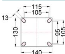
GPAX / FPAX larg. 4"
